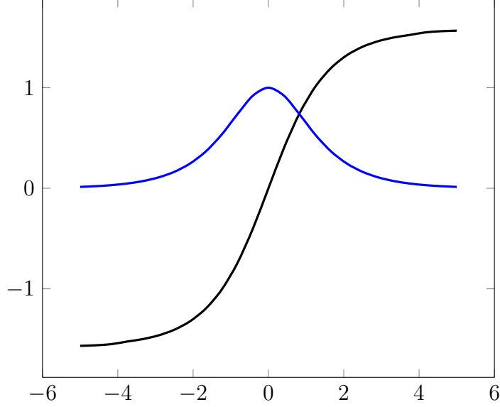
Figure 6: The sigmoid pair \text{sech}(x), \text{gd}(x)
