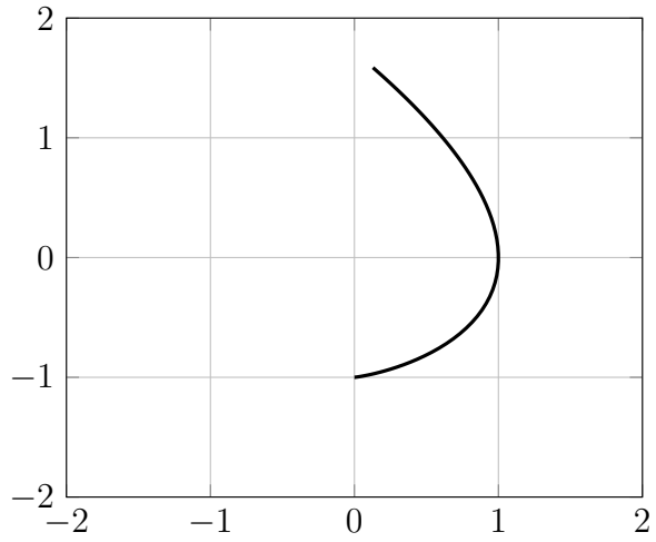
Figure 15: Parametric plot of t \mapsto \left( e^{1-t-e^{-t}}, e^{1-e^{-t}} - 1 \right)
