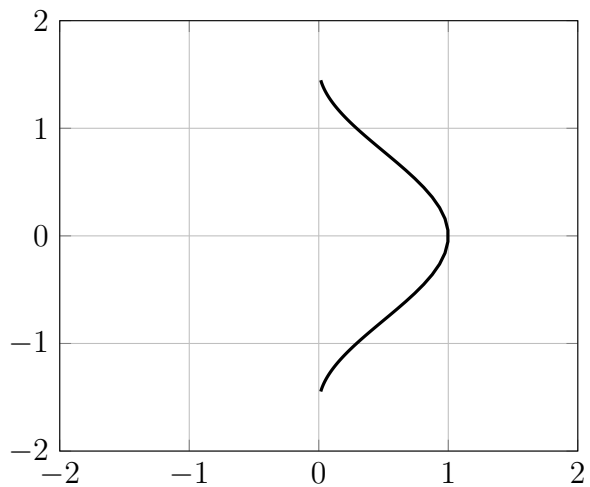
Figure 11: Parametric plot of t \mapsto \left(\frac{1}{1+t^2}, \tan^{-1}(t)\right)
