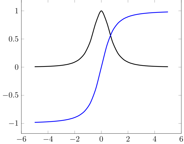
Figure 5: The sigmoid pair \frac{1}{(1+x^2)^{3/2}}, \frac{x}{\sqrt{1+x^2}}
