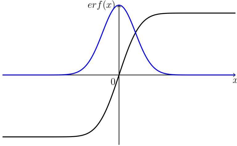
Figure 7: The sigmoid pair e^{-x^2}, \frac{\sqrt{\pi}}{2} \operatorname{erf}(x)
