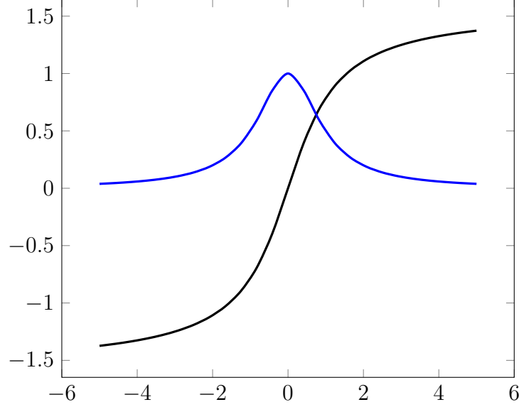
Figure 4: The sigmoid pair \frac{1}{1+x^2}, \tan^{-1}(x)
