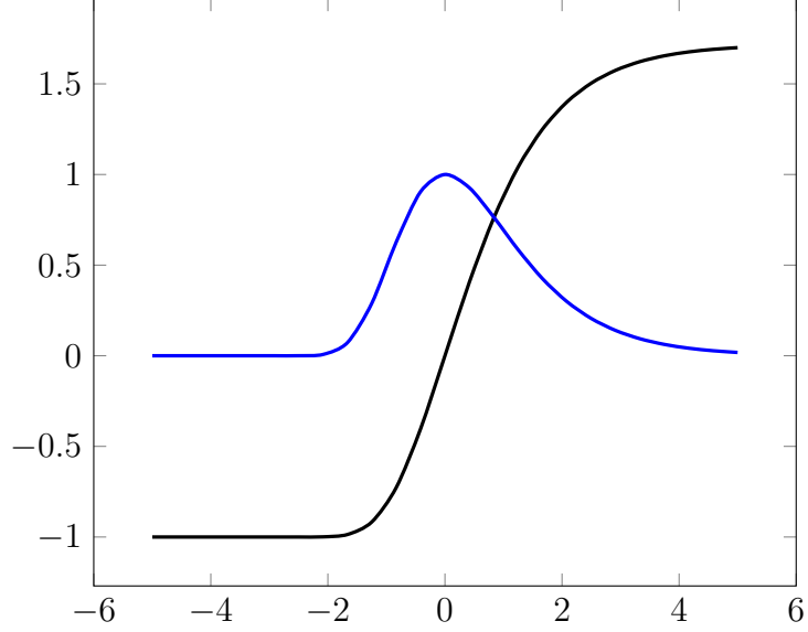
Figure 8: The Gompertz sigmoid pair e^{1-x-e^{-x}}, e^{1-e^{-x}} - 1
