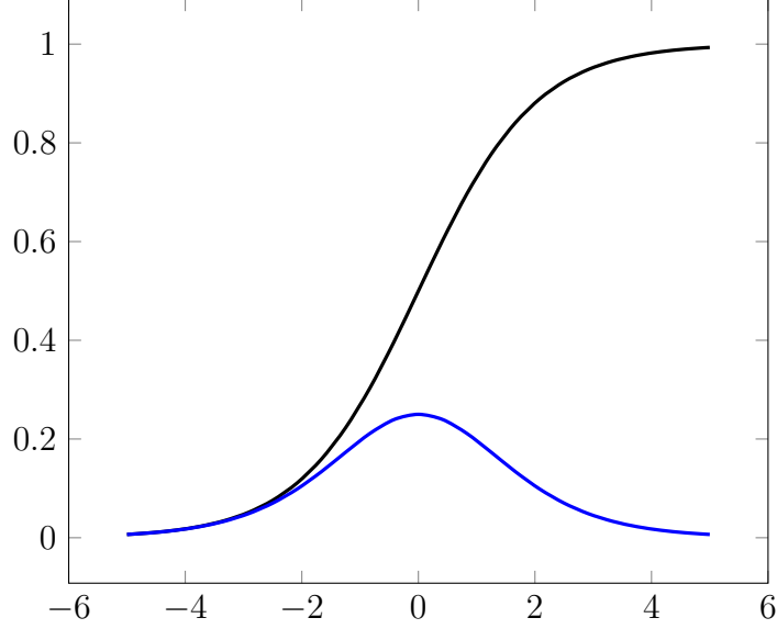
Figure 1: The sigmoid pair (\frac{1}{1+e^{-x}})', \frac{1}{1+e^{-x}}
