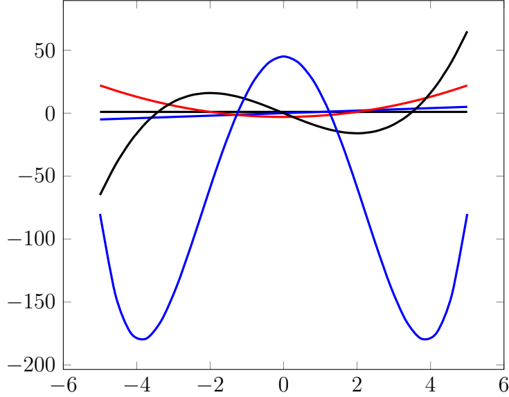
Figure 16: First five polynomials defined by the sigmoid array \left[ \frac{1}{(1+x^2)^{\frac{3}{2}}}, \frac{x}{(1+x^2)^{\frac{1}{2}}} \right]
