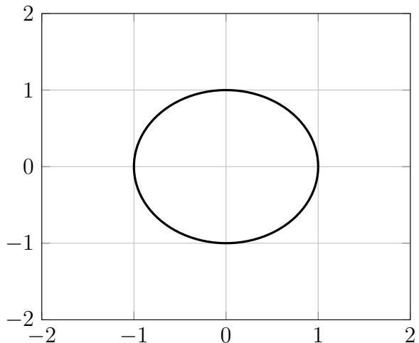
Figure 9: Parametric plot of t \mapsto (\cos(t), \sin(t))
