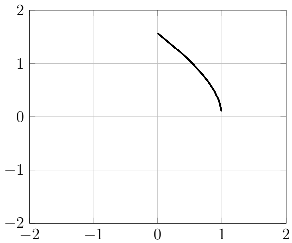
Figure 13: Parametric plot of t \mapsto (\operatorname{sech}(t), \operatorname{gd}(t))
