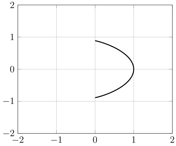
Figure 14: Parametric plot of t \mapsto \left( e^{-t^2}, \frac{\sqrt{\pi}}{2} \operatorname{erf}(t) \right)
