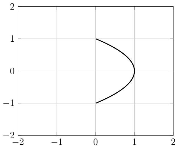
Figure 10: Parametric plot of t \mapsto (\operatorname{sech}^2(t), \tanh(t))
