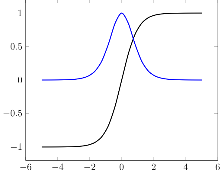
Figure 2: The sigmoid pair \text{sech}^2(x) , \tanh(x)
