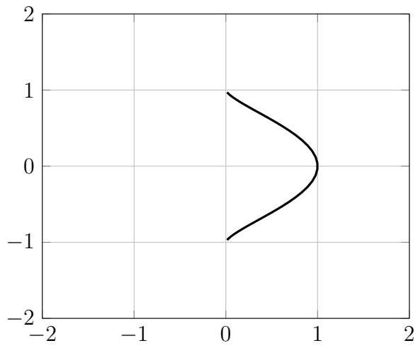
Figure 12: Parametric plot of t \mapsto \left( \frac{1}{(1+t^2)^{3/2}}, \frac{t}{(1+t^2)^{1/2}} \right)
